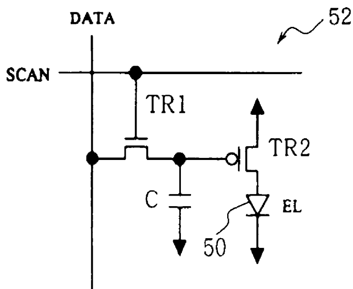
FIG. 51 PRIOR ART
